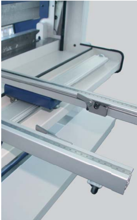
Optional: 2 variable gauge arms with scale, movable on linear guide incl. 2 tipping gauges
