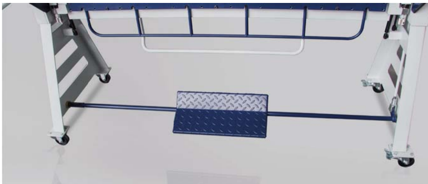
Optional: Tool case (picture above) Foot pedal for a fast opening and closing of the clamping beam (picture below)
